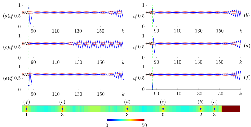
Figure 2. Finite-time stabilization of the unstable period-1 orbit using different control impulses as presented in the horizontal H-rank pattern. The colors of each line have the same meaning as in Figure 1. Each panel corresponds to the marking of trenches in the H-rank pattern. The digits below the markings depict the number of steps violating the tolerance corridor right after the control impulse. Panel (d) is an exact copy of Figure 1.
