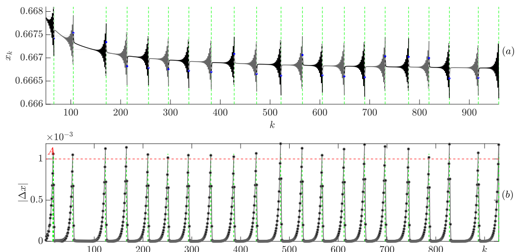
Figure 11. The adaptive continuous stabilization scheme of the unstable period-1 orbit of the fractional difference logistic map at A = 0.001 . Panel (a) displays the trajectory of the system (green vertical dashed lines denote the steps where the control impulse is used). Panel (b) displays the absolute differences of the adjacent points of the trajectory. The dashed red line in (b) indicates the threshold A for |\Delta x| = |x_k - x_{k-1}| . When this threshold is violated ( |\Delta x| > A ), a control impulse is applied.
