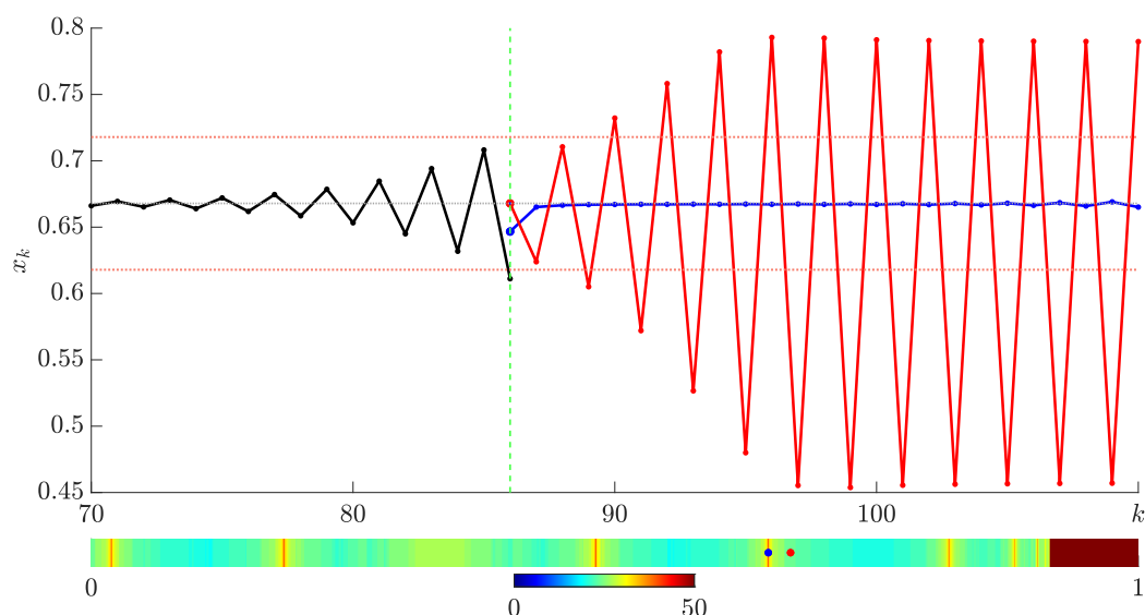
Figure 3. Comparison of the finite-time stabilization of the unstable period-1 orbit using the initial condition x_0 = 0.646674667466747 from Figure 2c versus the naive stabilization attempt using the unstable period-1 value x_* = 0.667893217185495 . In the top panel, the black line denotes the trajectory x before the stabilization step k = 86 , the red line denotes the the trajectory after naive stabilization, the blue line denotes the the trajectory after finite-time stabilization, the two red dotted lines denote the the tolerance corridor \delta = 0.1 , and the green vertical dashed line denotes the stabilization step k = 86 . The initial conditions for stabilization are marked with blue and red dots in the H-rank visualization in the bottom panel.
