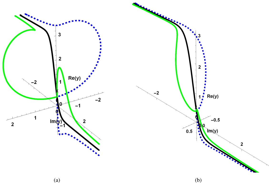
Figure 3. Solutions to the fractional Riccati equation (5.4). Initial conditions are set to x_0 = 0, u_0^{(0)} = 2/5 for both (a) and (b). The initial condition corresponding to the coefficients of the fractional series powers is set to v_1 = 5, v_1 = 1 in (a) and (b) respectively. The green solid line and blue dashed line denote solutions corresponding to different branches of \sqrt{x} . The black line corresponds to the non-fractional solitary solution (5.3).
